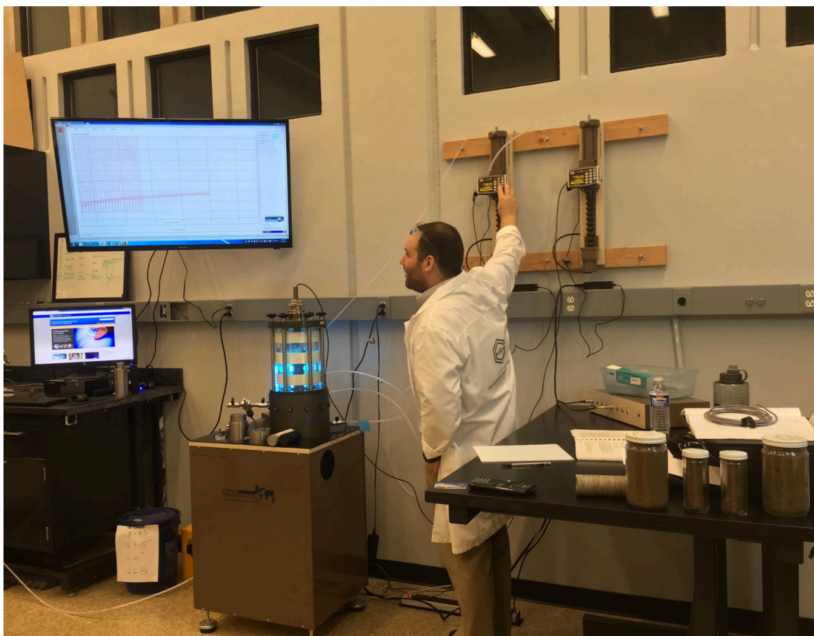
Figure 7: Cyclic Triaxial Machine at University at Buffalo
